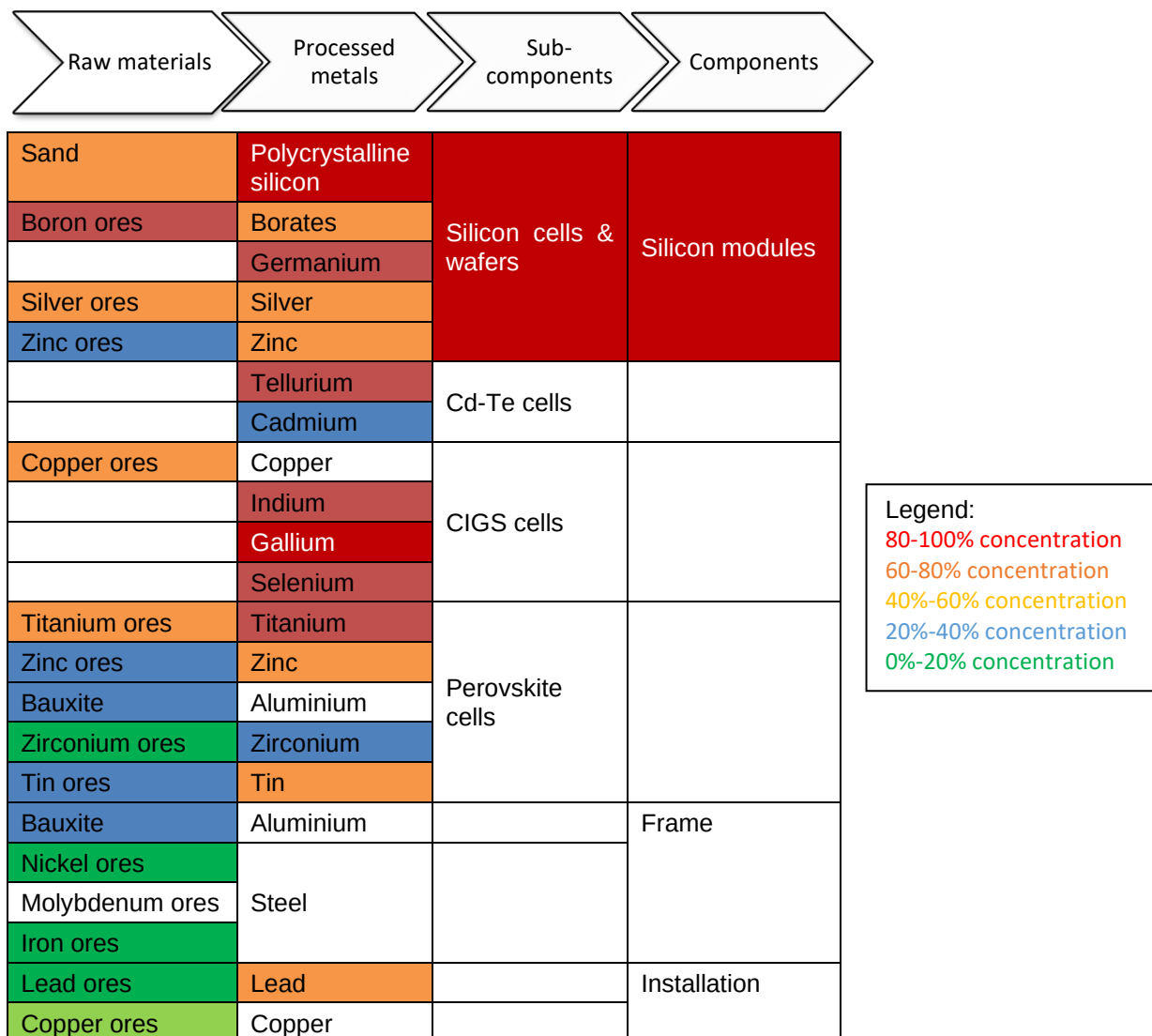
Figure 13: China's involvement in the supply chain for solar PV in 2022
