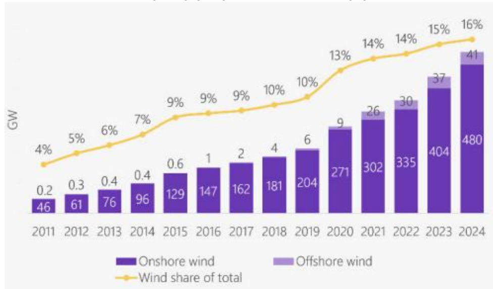
Figure 6: Total installed wind capacity (GW) and share of total (%)
