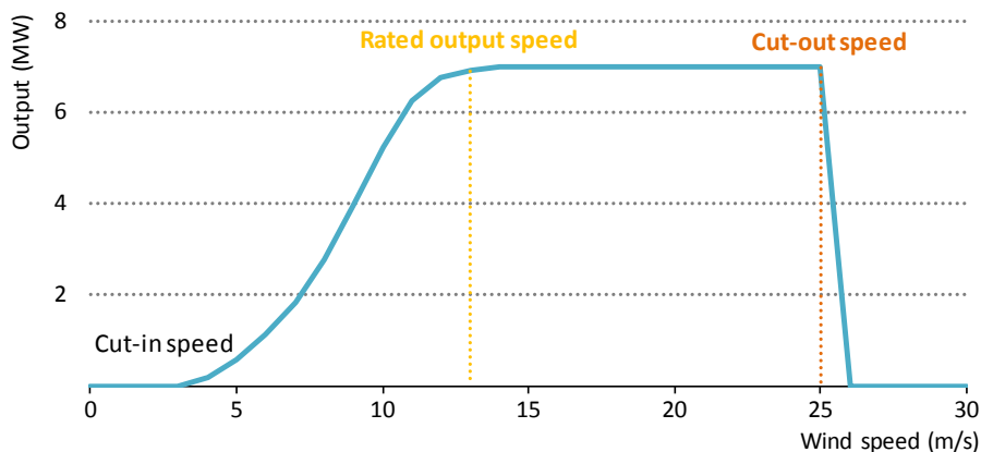
Figure B.1 ▶ Illustrative power curve for a 7 MW wind turbine
