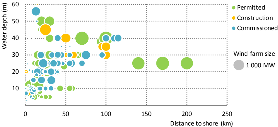
Figure B.4 ▶ Water depth and distance to shore for offshore wind projects
