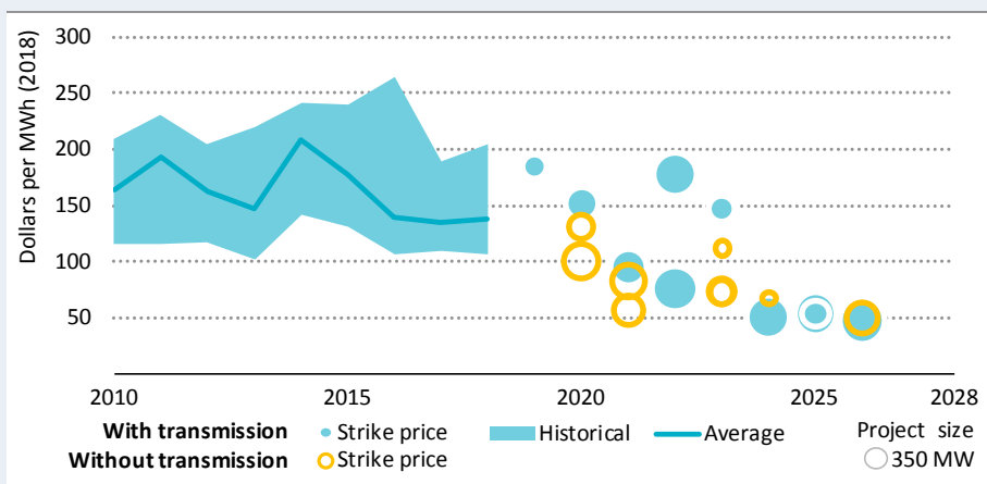
Figure 8 ▶ Historical LCOE of offshore wind and strike prices in recent auctions in Europe
