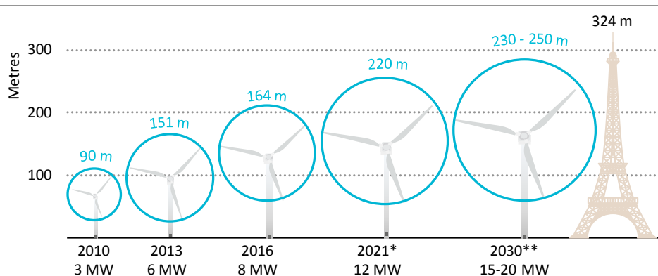
Figure 3 ▶ Evolution of the largest commercially available wind turbines
